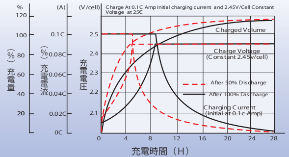
Charging Characteristics
